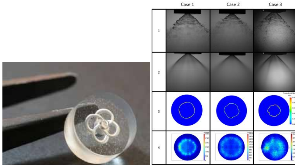
Figure 1. PSA with helical inlet (left). Findings for three manufactured atomizers operated at 3.34 g/s (right). 1st and 2nd row: instantaneous and average spray images, respectively. 3rd row: Computed normalized mass flux at a plane 0.7 mm downstream of the orifice exit. 4th row: the intensity of LIF signal taken 32 mm downstream of the orifice exit.
