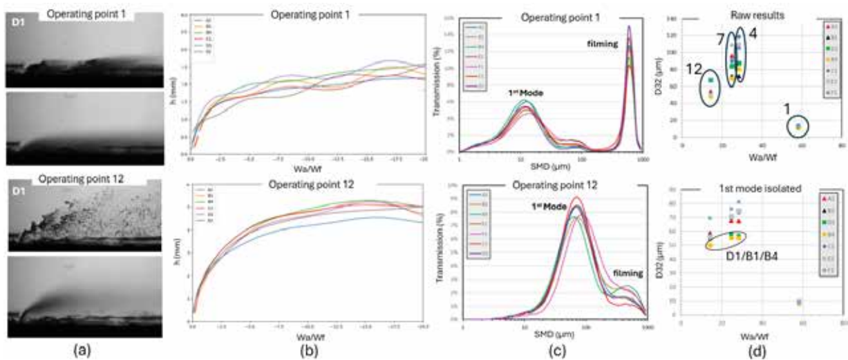
Figure 2. (a) Example of instantaneous (top) and time-averaged (bottom) shadowgraph images for configuration D1 and operating points 1 and 12, (b) Corresponding penetration curves and (c) Probability Density Function (PDF) with the 1 st mode and the filming mode identified for all configurations, (d) Sauter Mean Diameter (or D32) as a function of the W_a/W_f ratio considering all operating modes (top) and with the 1 st mode isolated (bottom)
