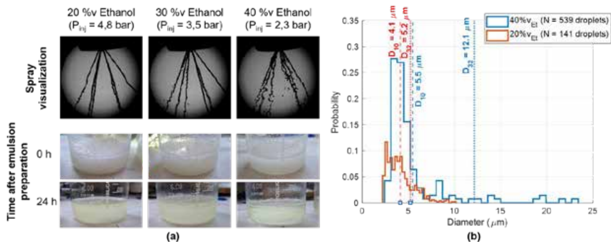
Figure 1. Results for ethanol-in-oil emulsion preparation: a) spray images (100 ml/min, high-speed shadowgraphy) and emulsion appearance at 0h and 24h after preparation, for ethanol-in -oil emulsions from 20 to 40 %v ethanol; b) probability density function of the ethanol droplet size for 40%v and 20%v ethanol content in the emulsion, including mean diameter ( D_{10} ) and Sauter mean diameter ( D_{32} ) values.
