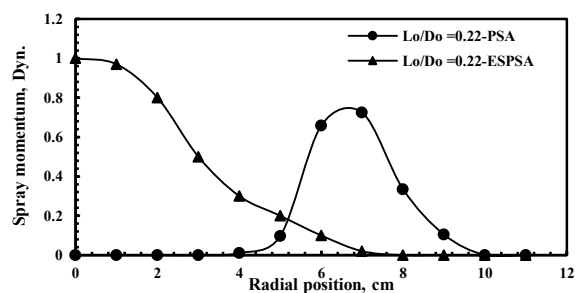
Fig. 8 Radial distribution of spray momentum for PSA and ESPSA at L_o/D_o = 0.22 , at P = 4 bar, W \times H = 1.5 \times 1.5 \text{ mm}^2 and L_s/D_s = 0.664 .
