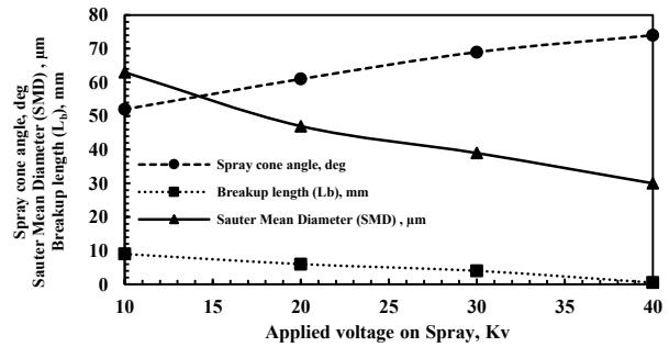
Fig. 6. Effect of Applied Voltage on the SCA, SMD and L_b of the ESPSA at fixed geometry.
