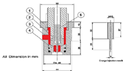
Fig. 1. Detailed dimensions of the Electrostatic Pressure Swirl Atomizer (ESPSA).
